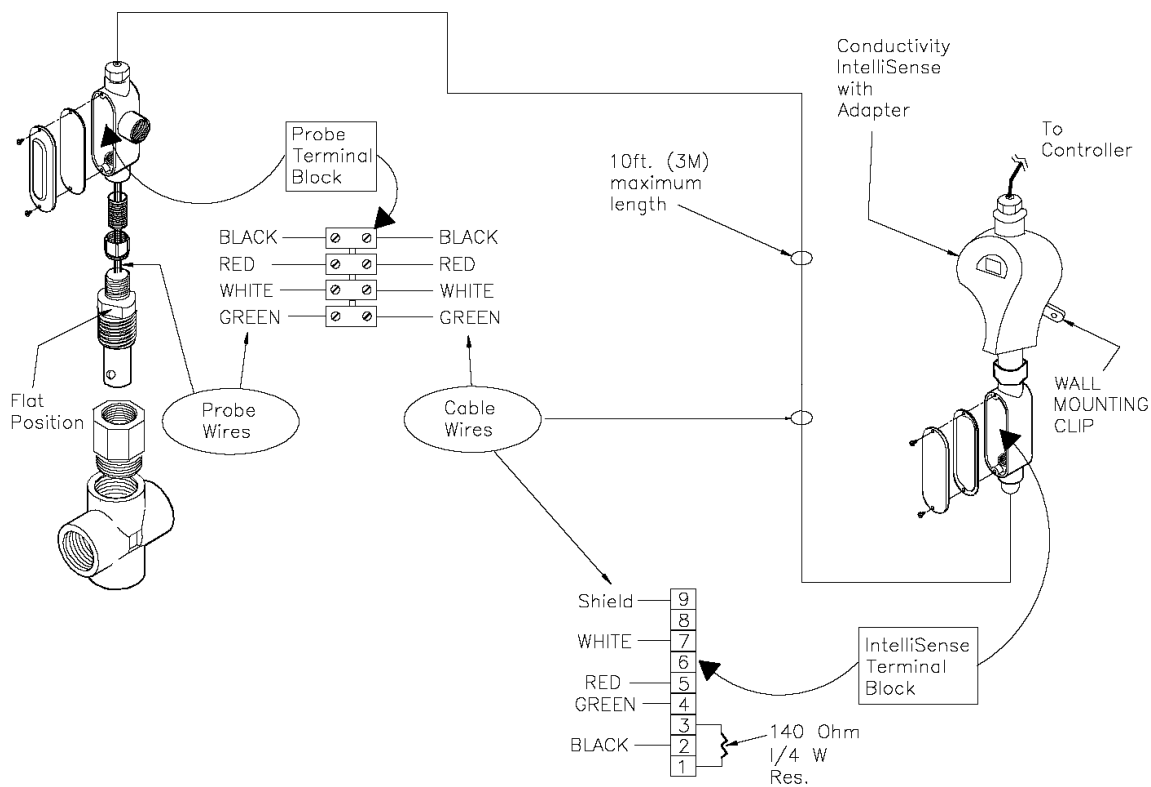
Fig. 6 Boiler probe
